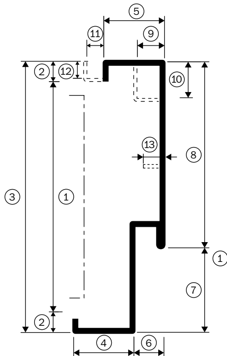
Bandseite (BS)
